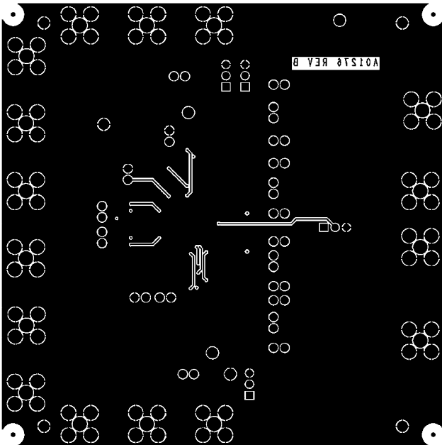
Figure 6. Wiring Side Copper
