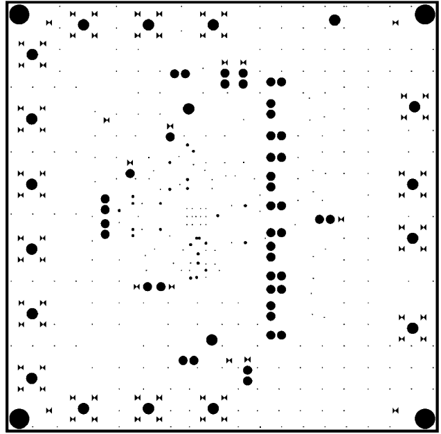
Figure 7. Inner Layer No. 1
