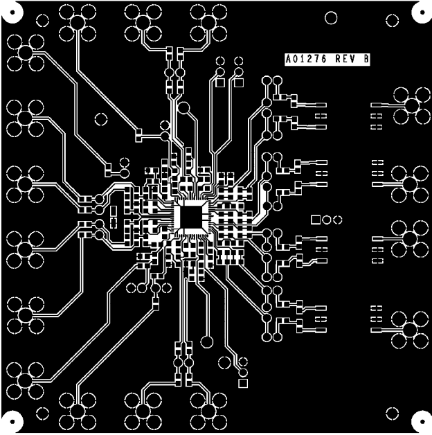
Figure 5. Component Side Copper
